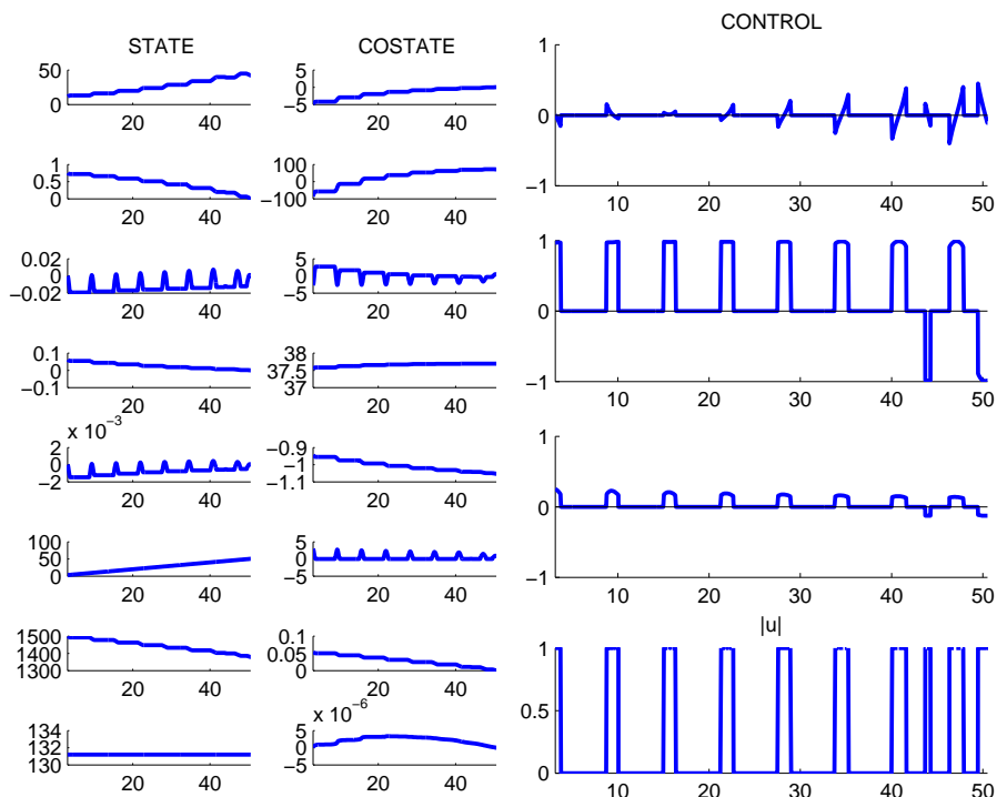
Orbital transfer (10N) - State, costate and control
